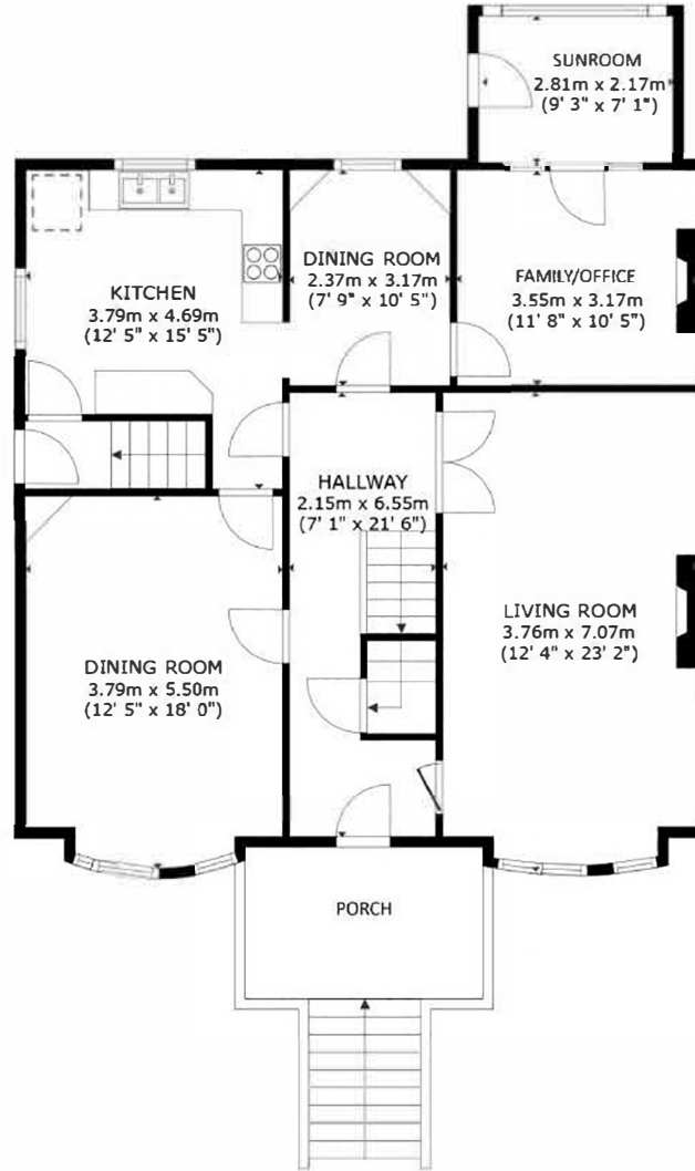
MAIN FLOOR
