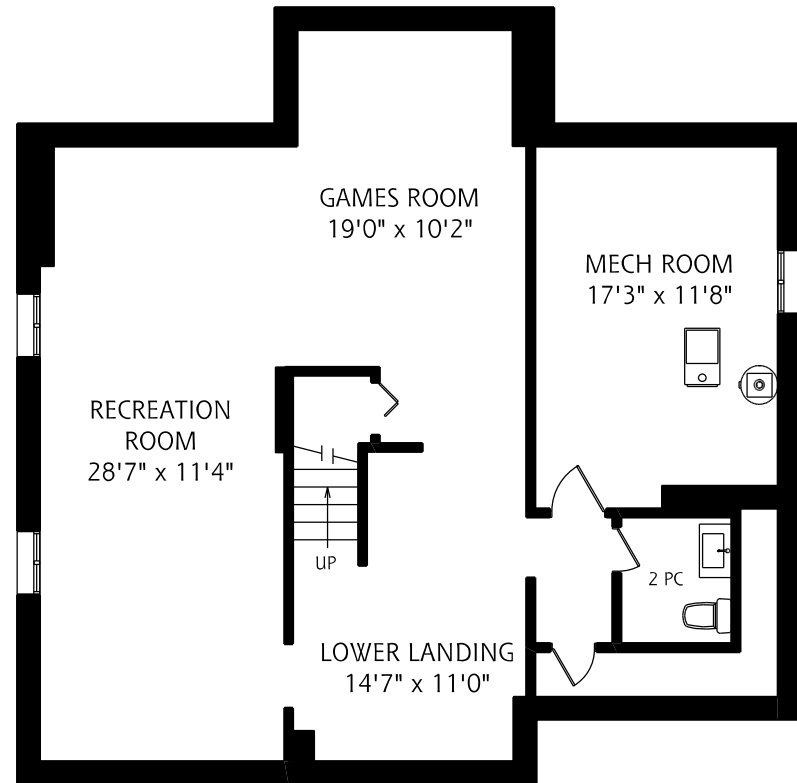
LOWER LEVEL 1,195 SQUARE FEET
