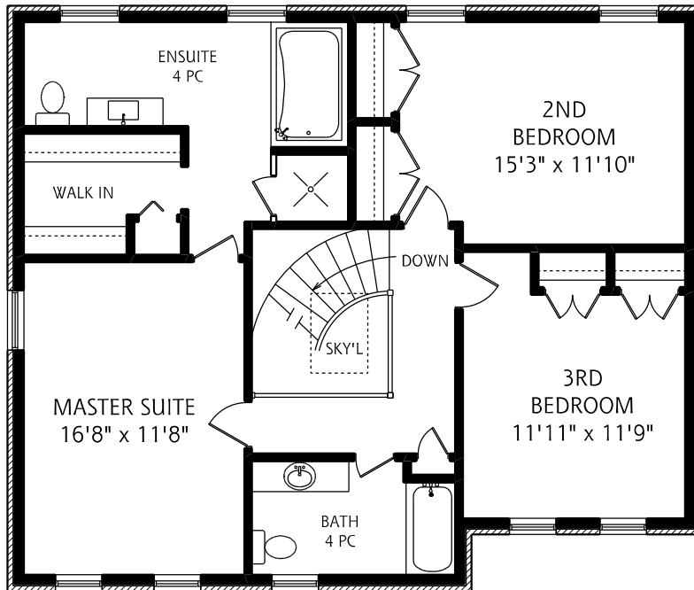
SECOND FLOOR 1,125 SQUARE FEET
