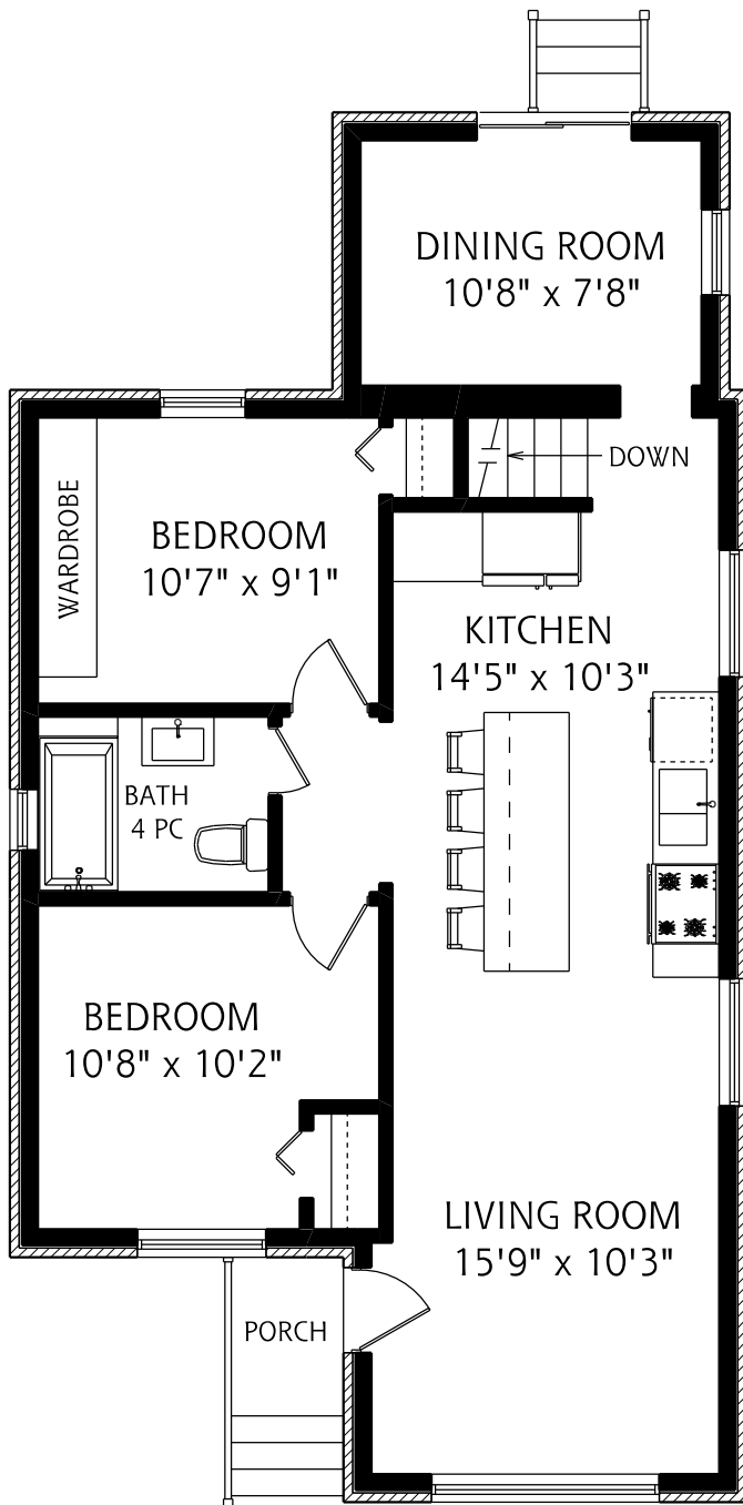
MAIN FLOOR 835 SQUARE FEET
